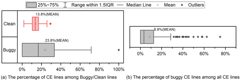
Fig. 3. The distribution of the ratios of CE lines (control elements) in all defective files of ActiveMQ-5.0.0.
