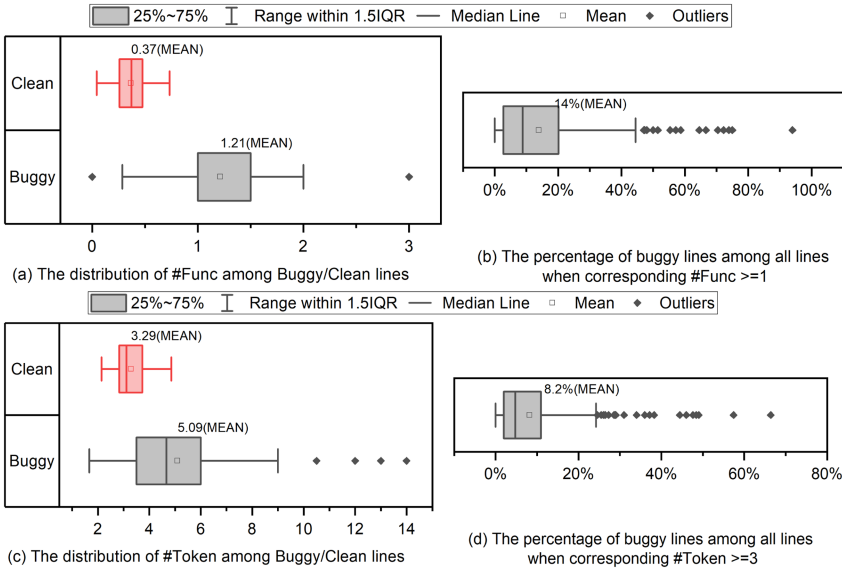
Fig. 4. The distribution of the number of function calls and code tokens in all defective files of ActiveMQ-5.0.0.
