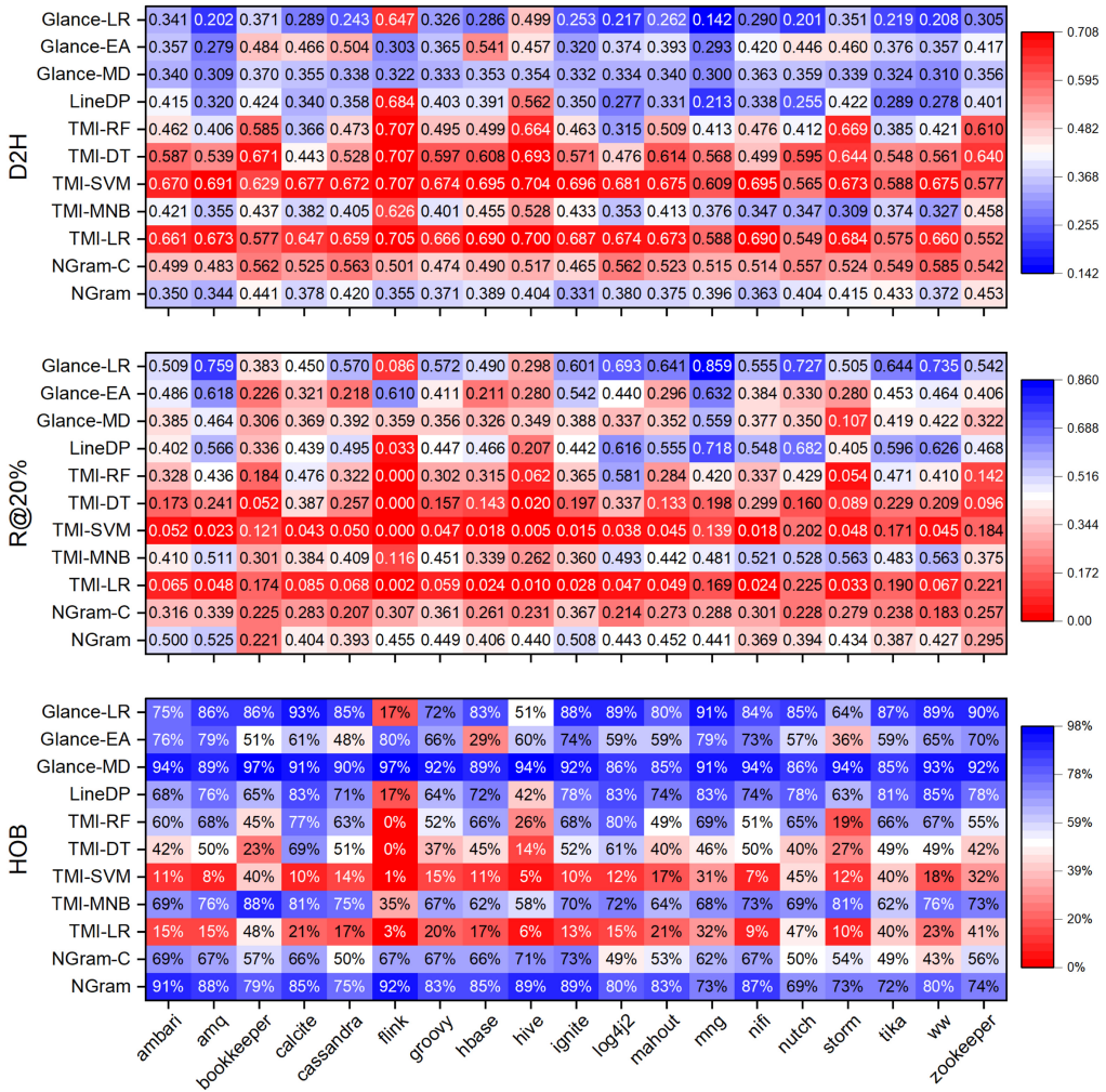
Fig. 11. Performance (D2H, R@20%, and HOB) comparison between NLPs, MITs, and GLANCE for each project.
