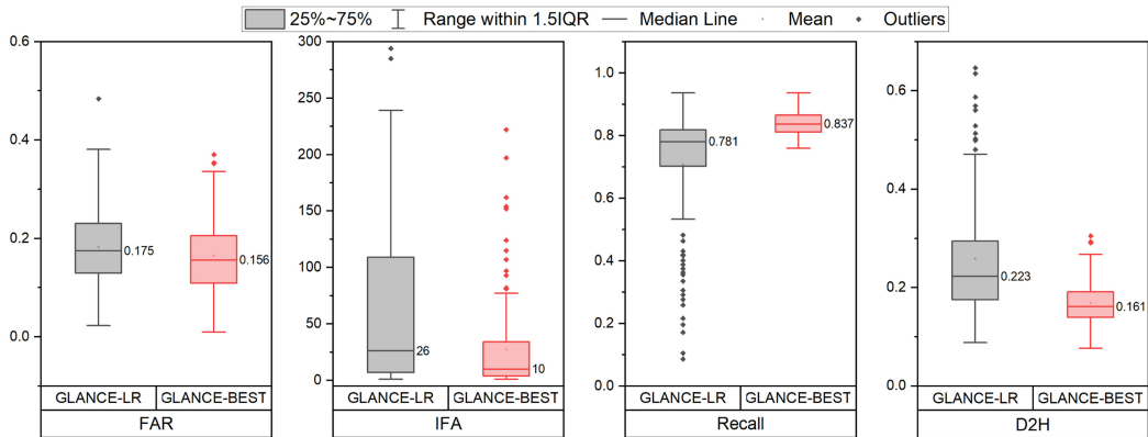
Fig. 20. The main performance comparison between GLANCE-LR and GLANCE-BEST.
