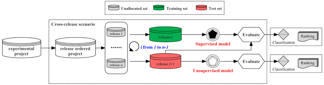
Fig. 9. Overview of the cross-release-prediction scenario.
