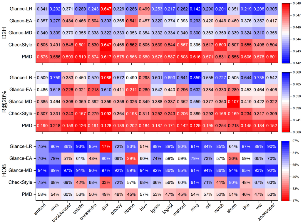
Fig. 13. Performance (D2H, R@20%, and HOB) comparison between SATs and GLANCE for each project.
