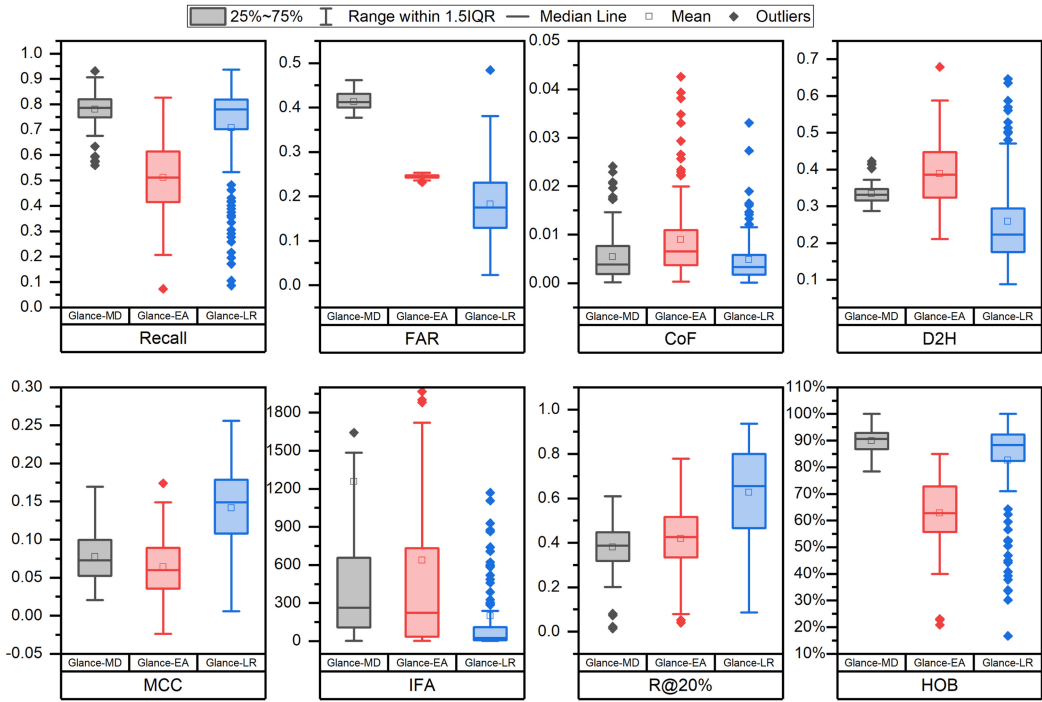
Fig. 10. Performance comparison among GLANCE-MD, GLANCE-EA, and GLANCE-LR.
