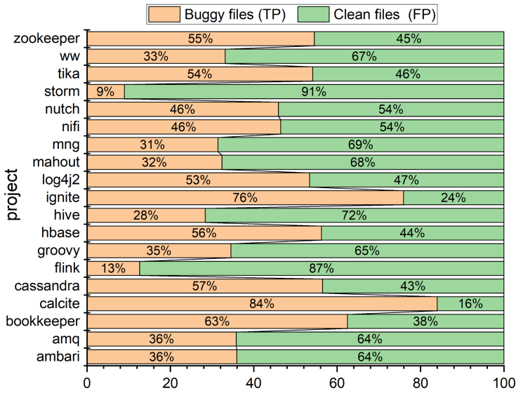
Fig. 19. The distributions of the real buggy files (TP) and the clean files (FP) in the set of defective files predicted by the file-level prediction model in GLANCE-EA.
