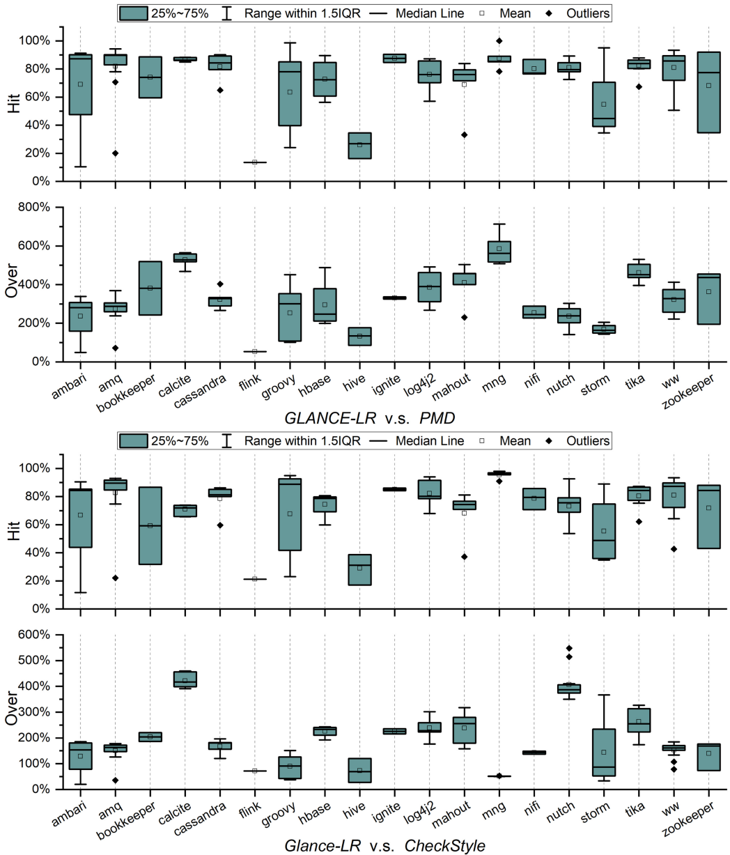
Fig. 14. The difference of buggy lines identification between PMD/CheckStyle and GLANCE-LR in individual projects.
