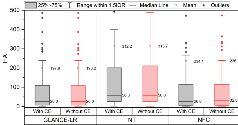
Fig. 18. The distributions of IFA values of GLANCE-LR, NT, and NFC with and without considering metric CE, respectively.
