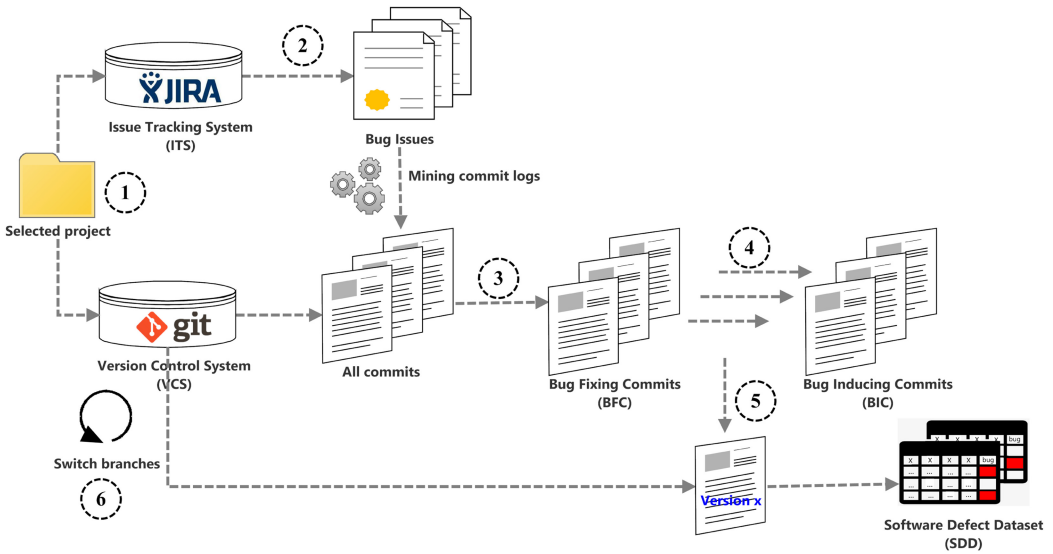
Fig. 7. The process of defect data collection for version x.
