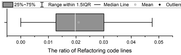
Fig. 22. The distribution of ratios of refactoring code lines detected by RefDiff among all BFC lines.
