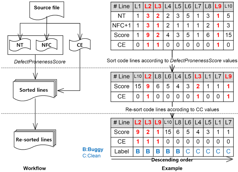
Fig. 6. An example for sorting lines in a defective file (The red number denotes that the line contains a control element, i.e., CE = 1).
