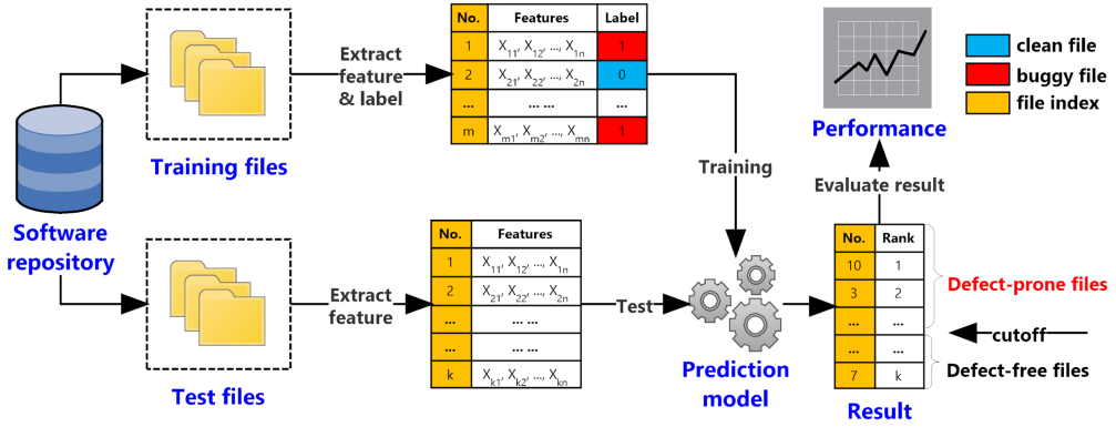
Fig. 1. General process of file-level defect prediction.
