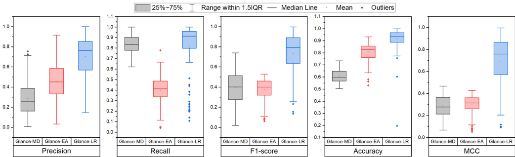
Fig. 15. The classification performance comparison between different file-level classifiers ( Precision = TP/(TP + FP) , Recall = TP/(TP + FN) , F1-Score = 2 \times Precision \times Recall/(Precision + Recall) , Accuracy = (TP + TN)/(TP + TN + FP + FN) ).
