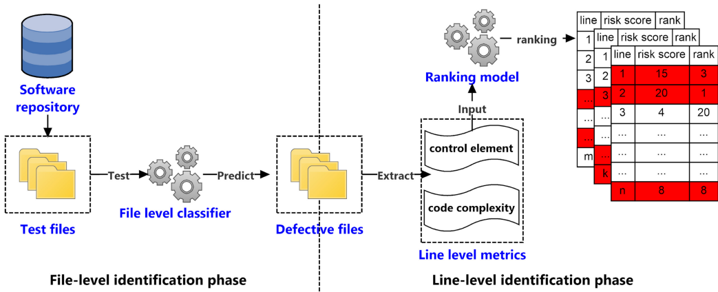
Fig. 5. The workflow of GLANCE.
