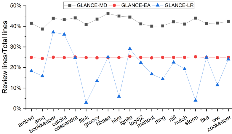
Fig. 16. The review effort (measured by SLOC) comparison between different file-level classifiers.
