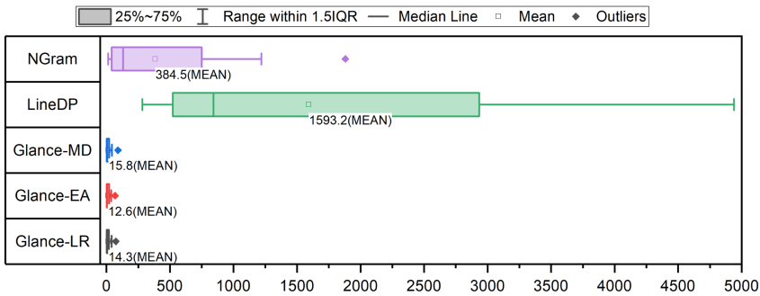
Fig. 21. The comparison of overall (building + prediction) time (Unit: second) between NGram, LineDP, and GLANCE.
