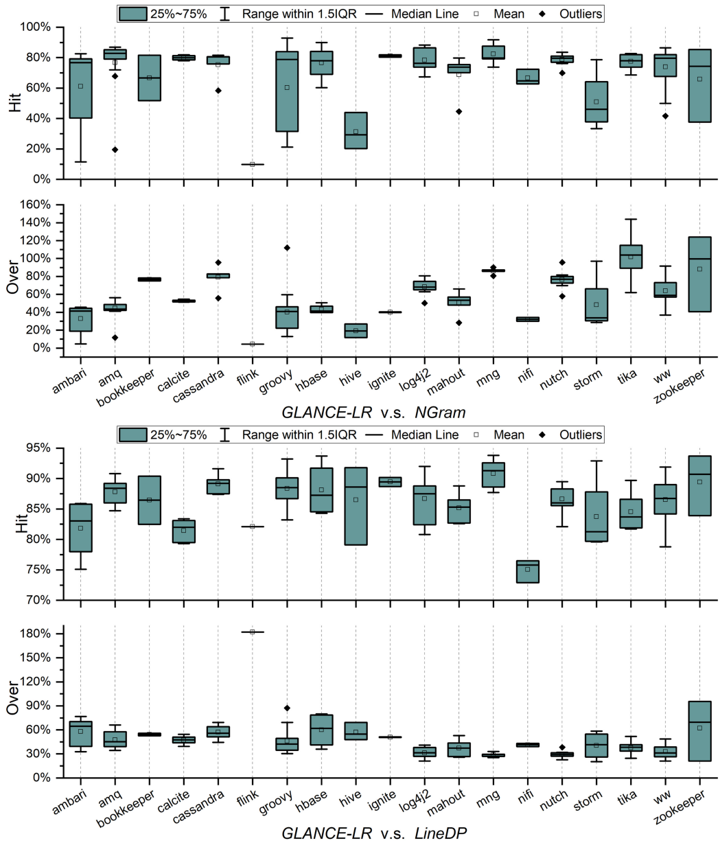
Fig. 12. The difference of buggy lines identification between NGram, LineDP, and GLANCE-LR in individual projects.
