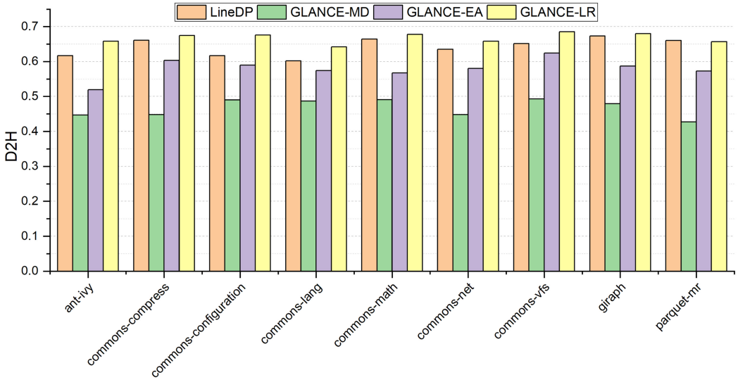
Fig. 23. The performance comparison between LineDP and GLANCE approaches in terms of D2H on JIT-Defects4J.
