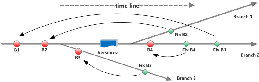
Fig. 8. Labeling the versions that are affected by a bug.
