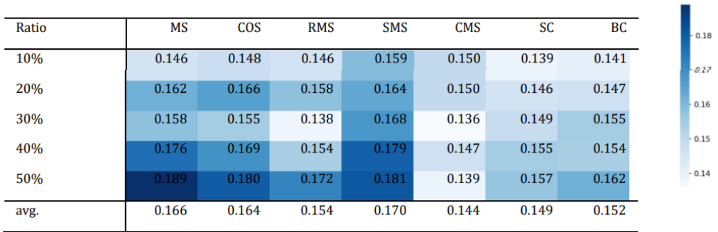
Fig. 3. (RQ5) The average Kendall's Tau on all used bugs of seven metrics by 10%–50% sampling ratio.
