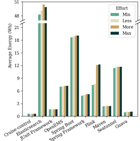
Figure 1: Average energy consumption per project across SpotBugs effort levels.
