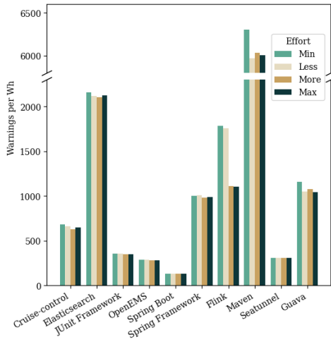
Figure 2: Number of warnings divided by energy consumption per project per effort
